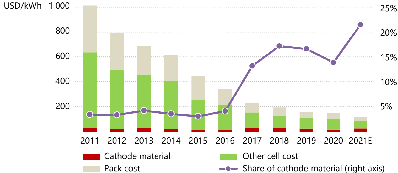
Average pack price of lithium-ion batteries and share of cathode material cost
